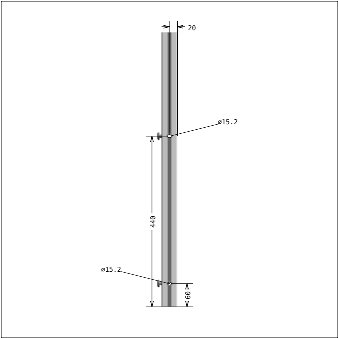
DRAWING 11, Pos 15 SIDE 1, bar length: 709.0 mm
