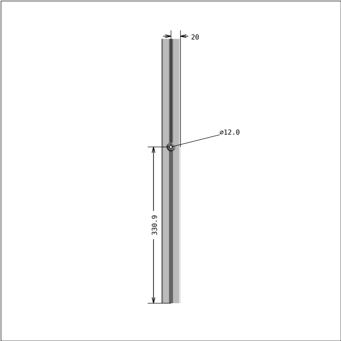
DRAWING 1, Pos 2 SIDE 1, bar length: 559.8 mm
