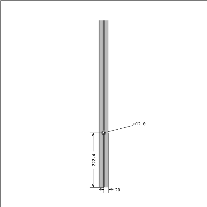
DRAWING 5, Pos 6 SIDE 1, bar length: 681.0 mm
