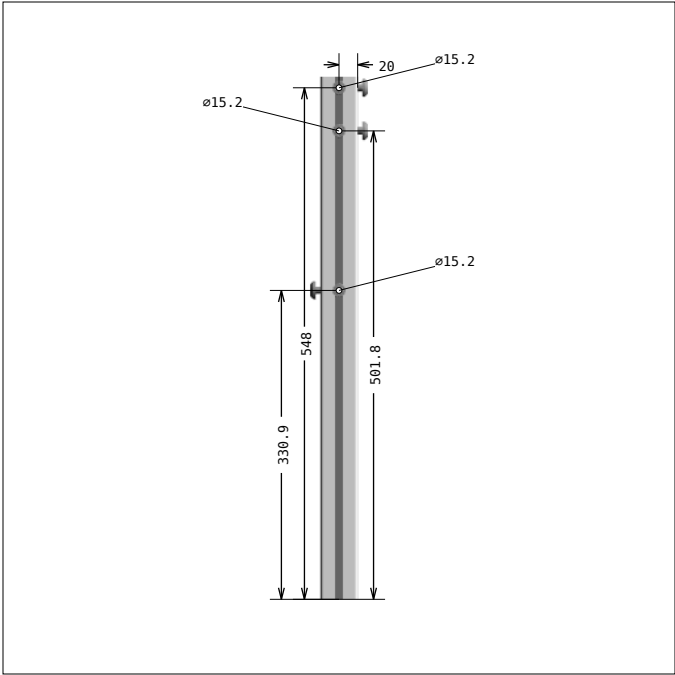
DRAWING 1, Pos 2 SIDE 4
