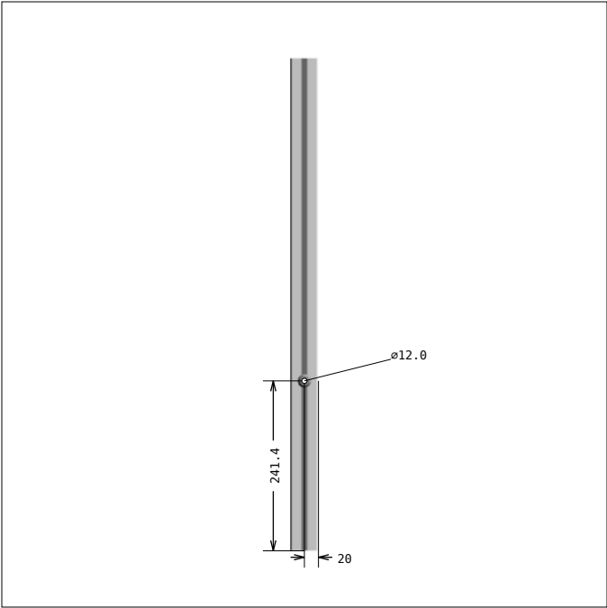
DRAWING 6, Pos 7 SIDE 3
