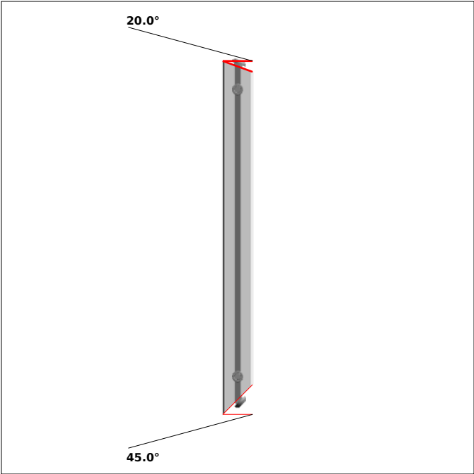
DRAWING 10, Pos 12 SIDE 1, bar length: 474.2 mm
