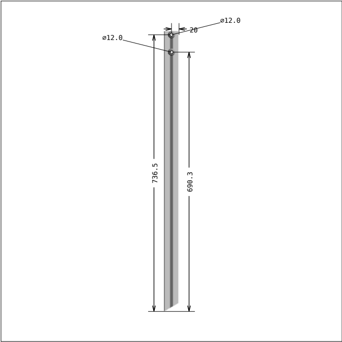
DRAWING 8, Pos 9 SIDE 3
