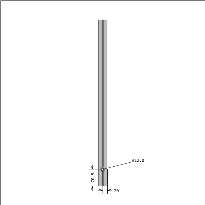
DRAWING 6, Pos 7 SIDE 1, bar length: 700.0 mm
