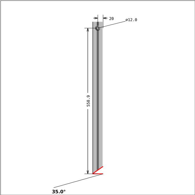
DRAWING 4, Pos 5 SIDE 1, bar length: 575.0 mm
