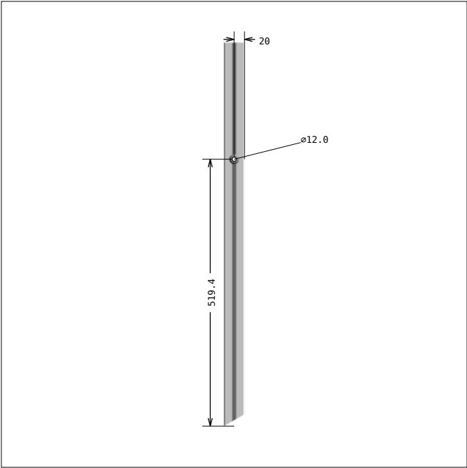
DRAWING 7, Pos 8 SIDE 3
