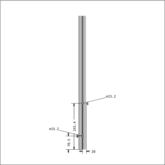
DRAWING 6, Pos 7 SIDE 4
