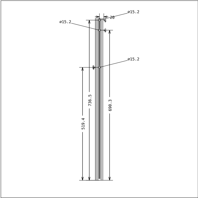
DRAWING 8, Pos 9 SIDE 4
