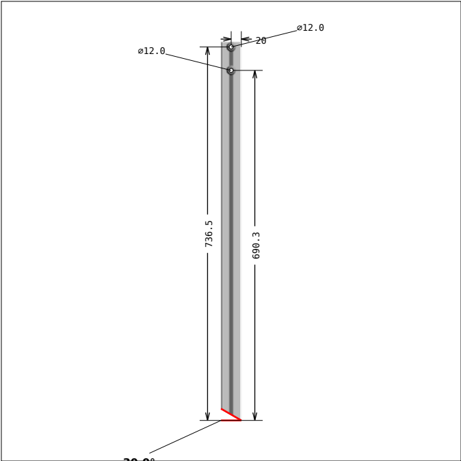
DRAWING 7, Pos 8 SIDE 1, bar length: 746.4 mm
