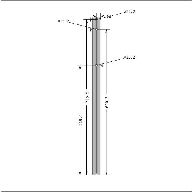
DRAWING 7, Pos 8 SIDE 4
