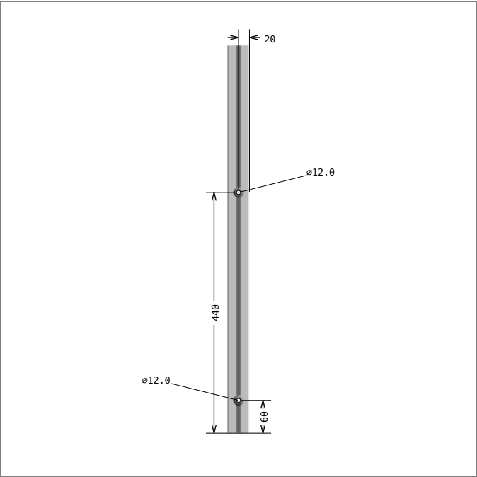
DRAWING 11, Pos 15 SIDE 2
